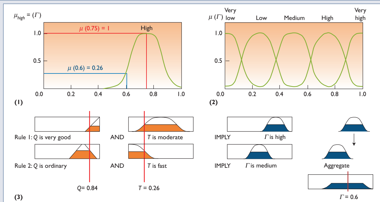
Figure A. Fuzzy membership functions and the fuzzy reputation aggregation procedure. We show (1) the high membership function of a local score ( \Gamma ), (2) the five levels of membership functions of \Gamma , and (3) the application of two rules to induce the seller's local score.
