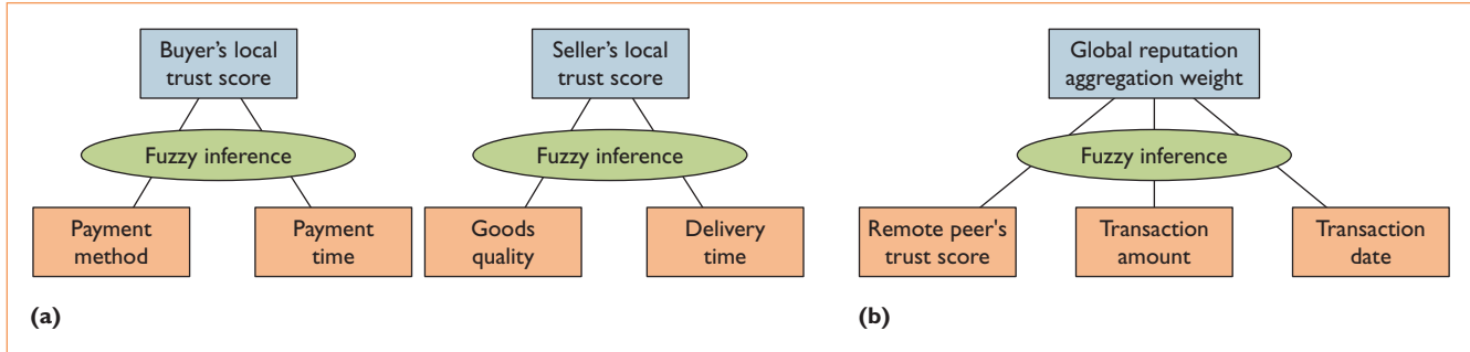
Figure 3. Local trust inference versus global reputation aggregation. The FuzzyTrust system (a) performs fuzzy logic inferences to determine the local trust scores and (b) uses accumulated local scores for weight inference in global reputation aggregation.
