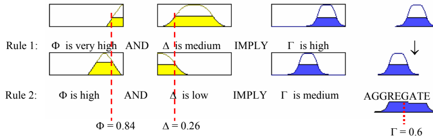
Fig. 5. Fuzzy logic inference between job success rate \Phi and self-defense capability \Delta to induce the trust index \Gamma of a resource site
